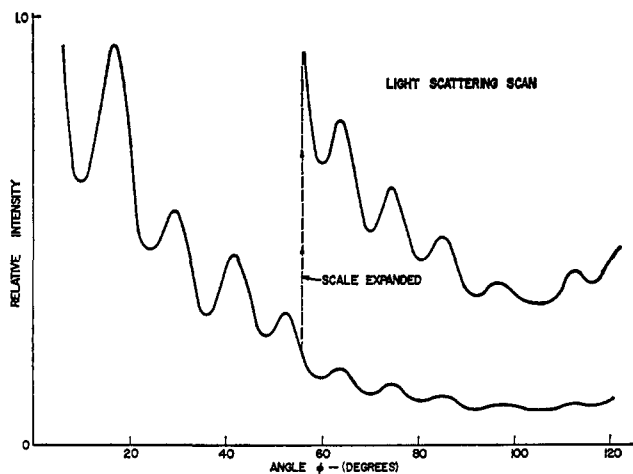
Figure 10. Photometer scan from monolayer film of 3.0- \mu poly(vinyltoluene) latex particles inclined at \theta_1 = 60^\circ (source, Hg vapor lamp with filter to give monochromatic light at 5460 \text{\AA} ).
