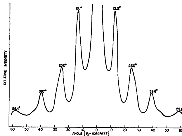
Figure 11. Photometer scan from same monolayer film as in Figure 10, but at normal incidence (source, He-Ne laser at 6328 \text{\AA} ).
